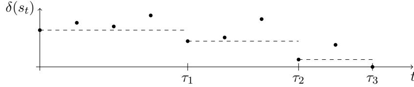
Figure 2: Phases in the proof of Lemma 14.3.
